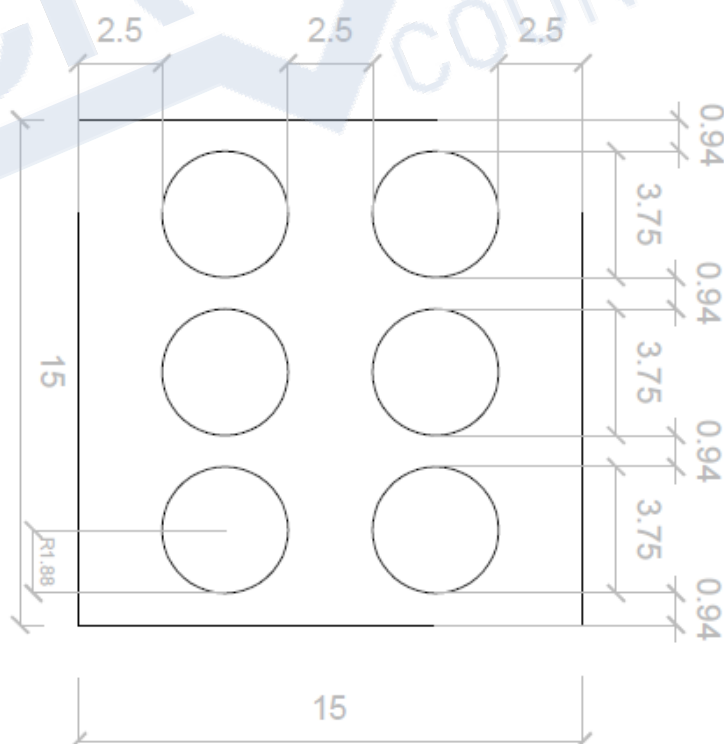
Figure 1: Dimensions (in cm) of the template used for the tile template measurement method
